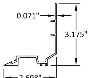
15 INTERLOCK ADAPTER
