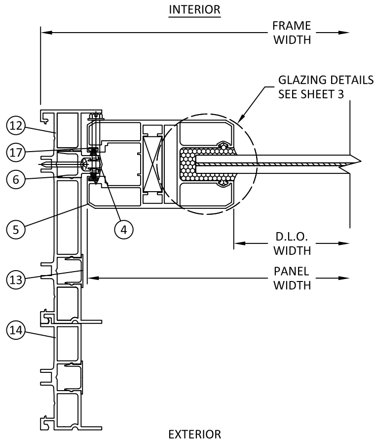
J 7 HORIZONTAL SECTION 3-TRACK JAMB FIXED PANEL
