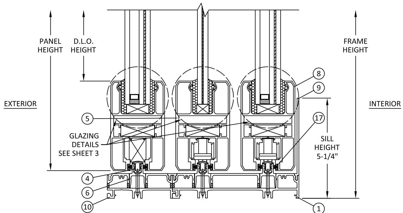
D 5 VERTICAL SECTION 3-TRACK SILL
