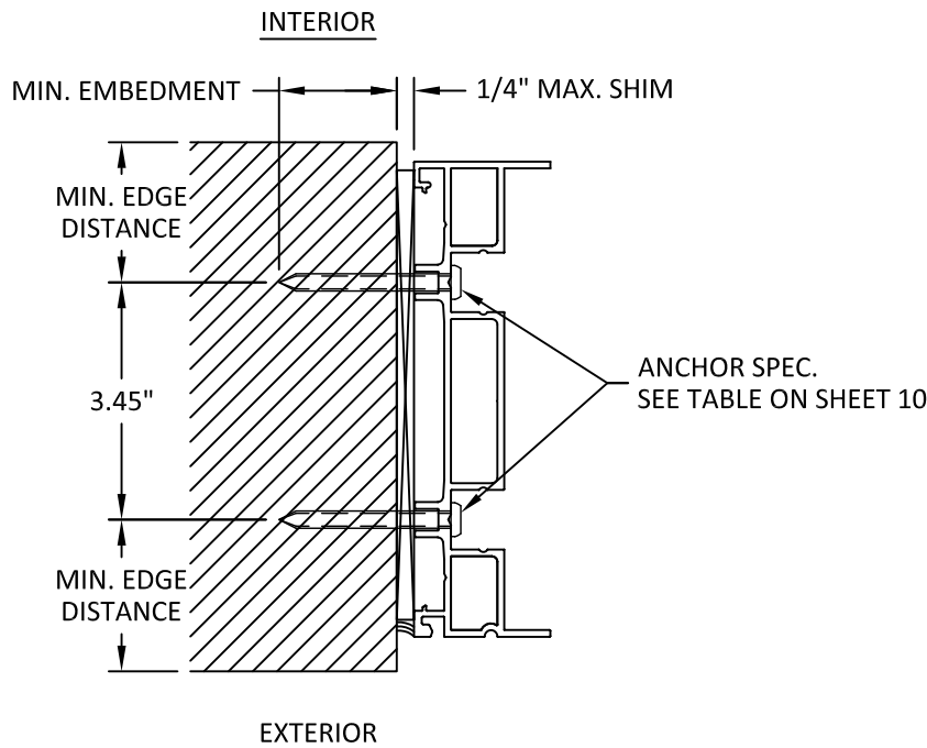
Q 9 INSTALLATION DETAIL 2-TRACK JAMB
