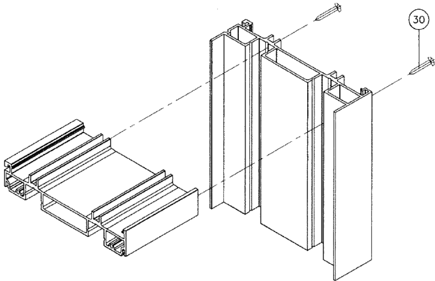
FRAME CORNER DETAIL 2 TRACK FRAME
