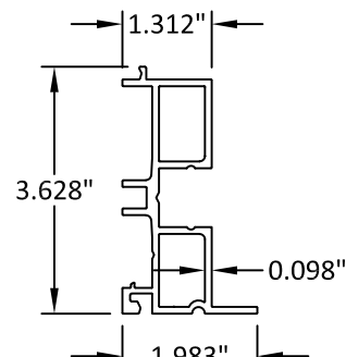
14 3/4 TRACK ADAPTER JAMB
