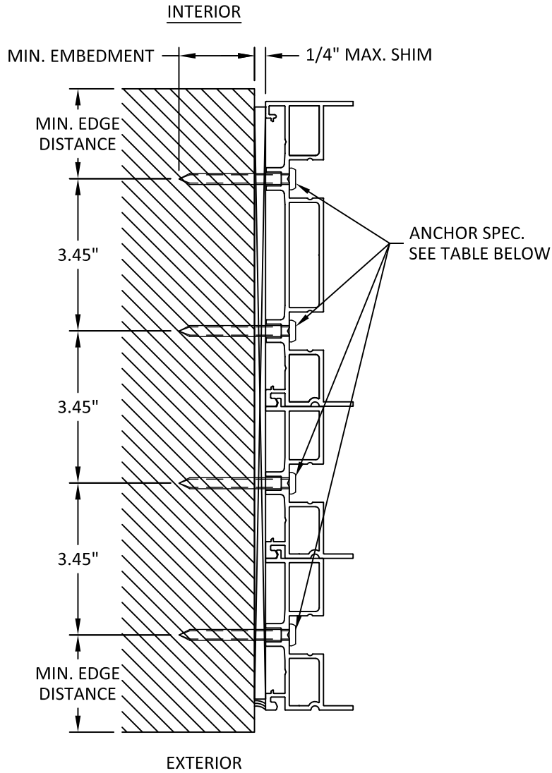
T 10 INSTALLATION DETAIL 4-TRACK JAMB
