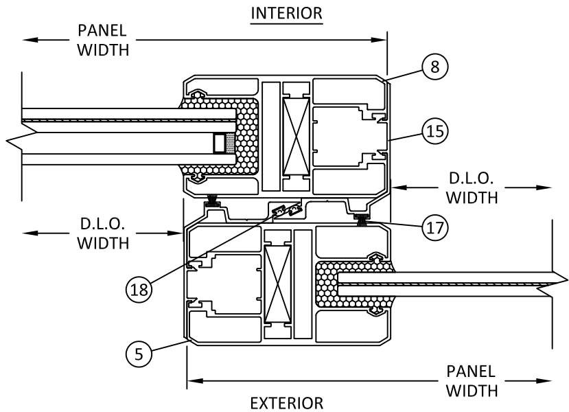
M 8 HORIZONTAL SECTION INTERLOCK
