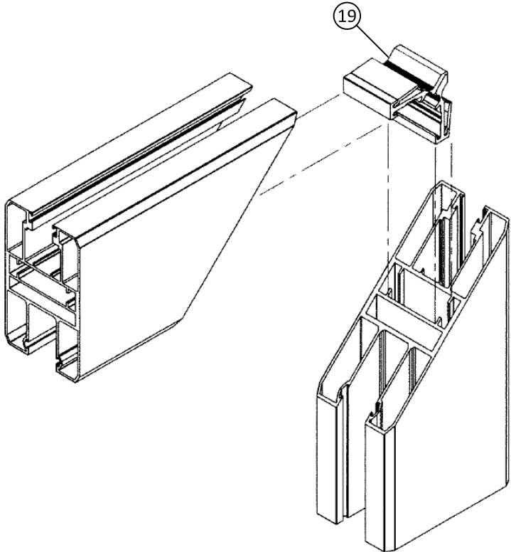
PANEL CORNER DETAIL
