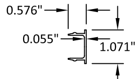
13 JAMB COVER
