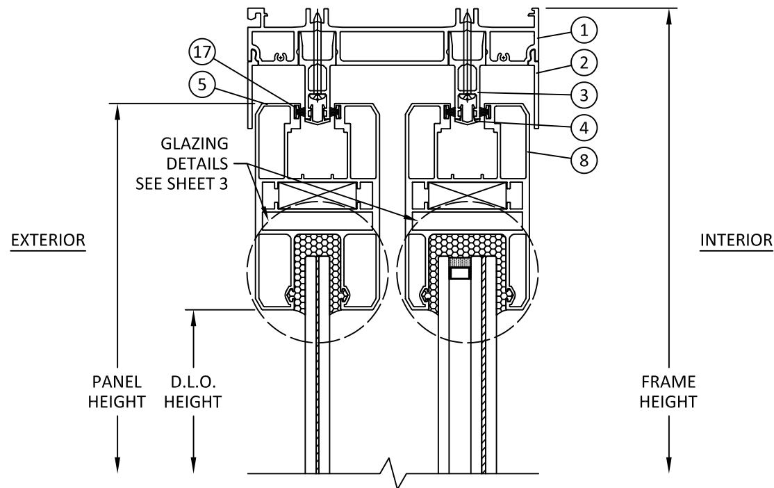
A 5 VERTICAL SECTION 2-TRACK HEAD
