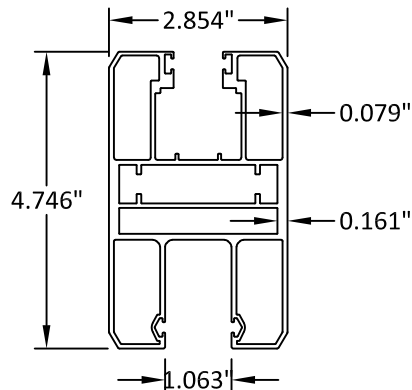
5 PANEL RAIL/STILE (MONO.)
