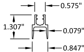
6 JAMB/SILL TRACK
