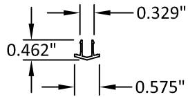
4 H/J/S TRACK COVER
