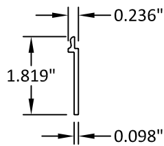
2 HEAD LEG EXTENSION
