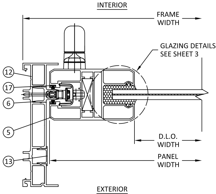
G 7 HORIZONTAL SECTION 2-TRACK JAMB OPERABLE PANEL
