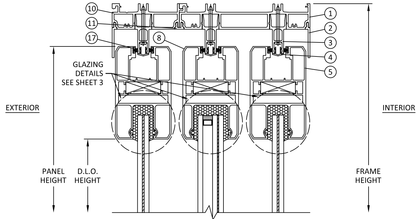
C 5 VERTICAL SECTION 3-TRACK HEAD
