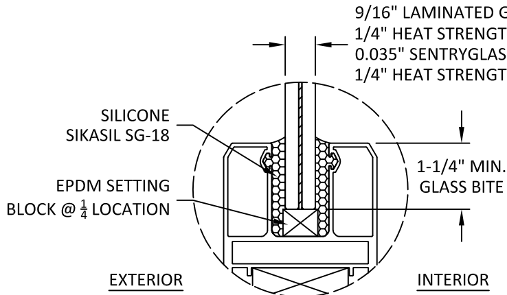
GLAZING DETAIL A SMALL MISSILE IMPACT
