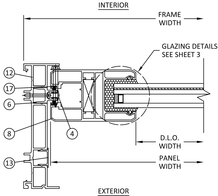
H 7 HORIZONTAL SECTION 2-TRACK JAMB FIXED PANEL
