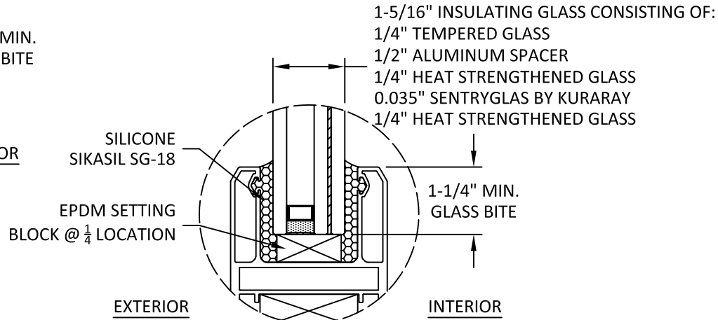
GLAZING DETAIL B SMALL MISSILE IMPACT
