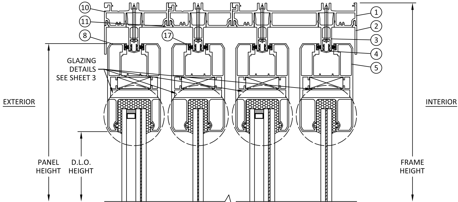
E 6 VERTICAL SECTION 4-TRACK HEAD
