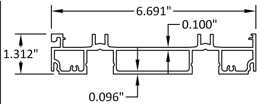
1 2 TRACK FRAME HEAD/SILL
