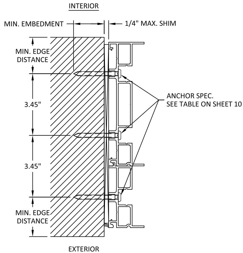
R 9 INSTALLATION DETAIL 3-TRACK JAMB
