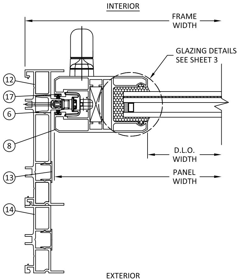
I 7 HORIZONTAL SECTION 3-TRACK JAMB OPERABLE PANEL
