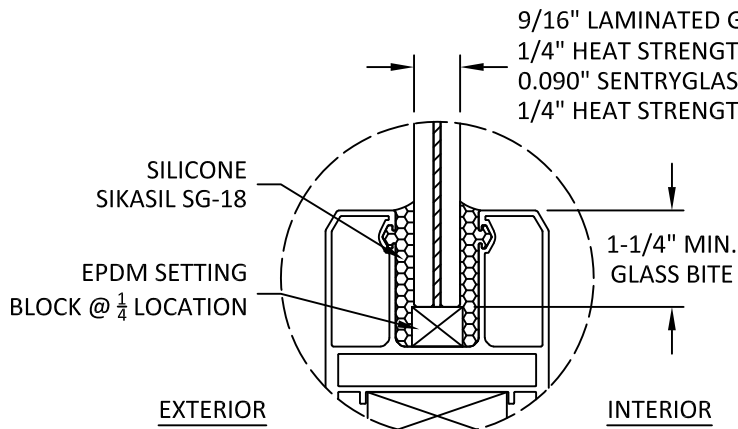
GLAZING DETAIL C LARGE MISSILE IMPACT
