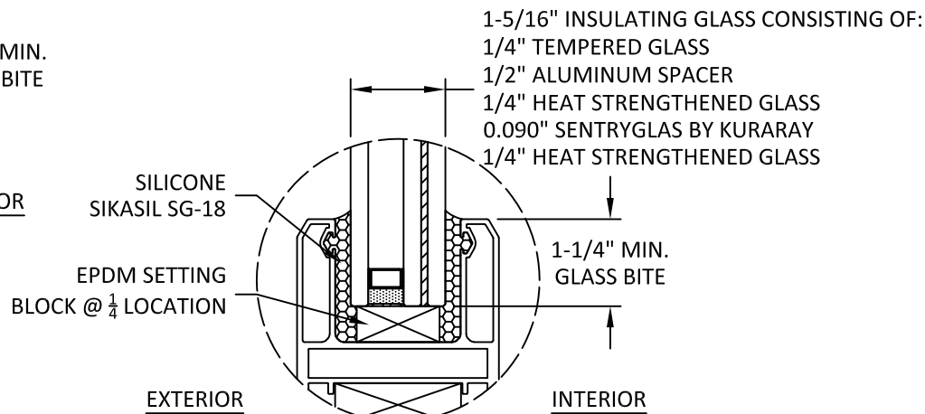
GLAZING DETAIL D LARGE MISSILE IMPACT
