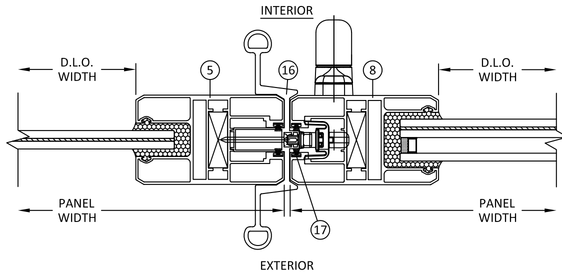
N 8 HORIZONTAL SECTION ASTRAGAL
