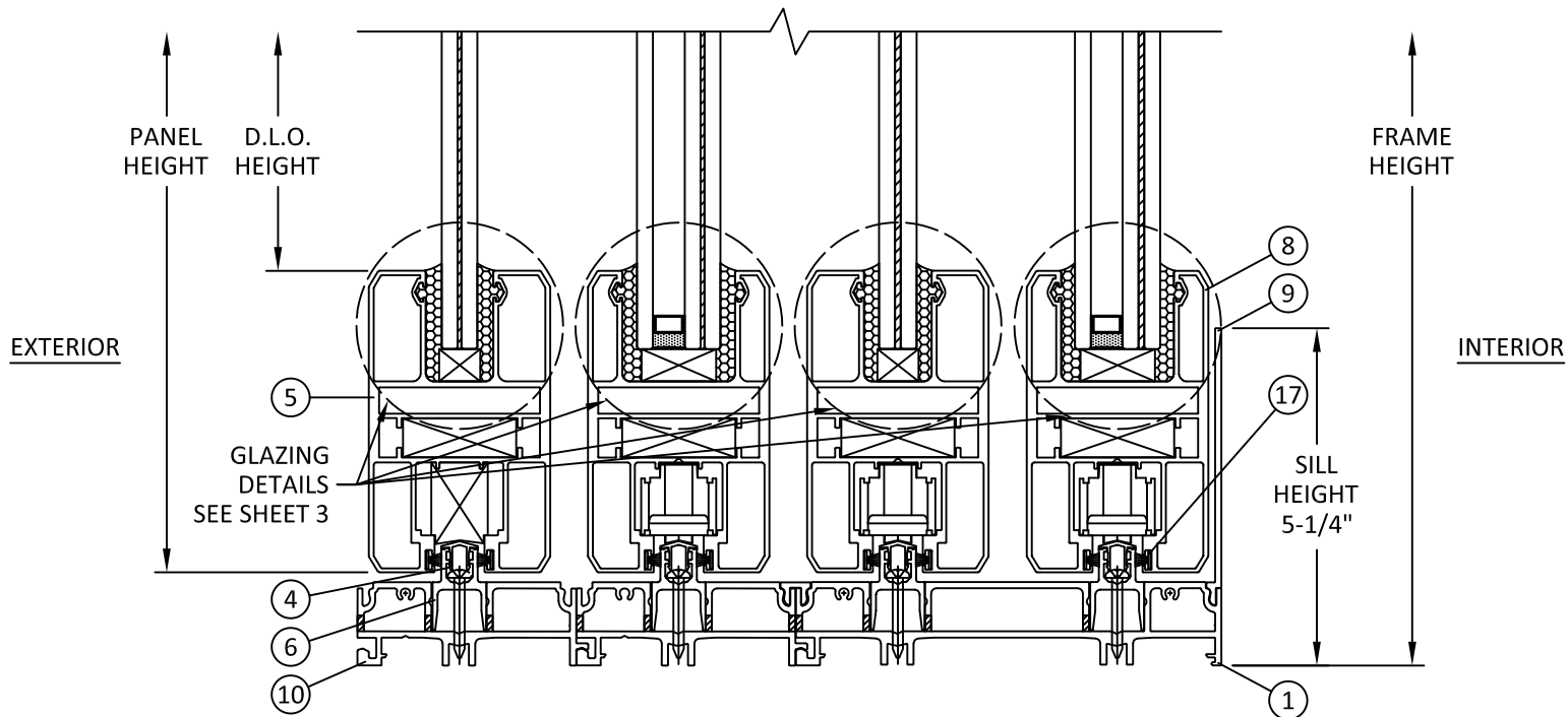
F 6 VERTICAL SECTION 4-TRACK SILL
