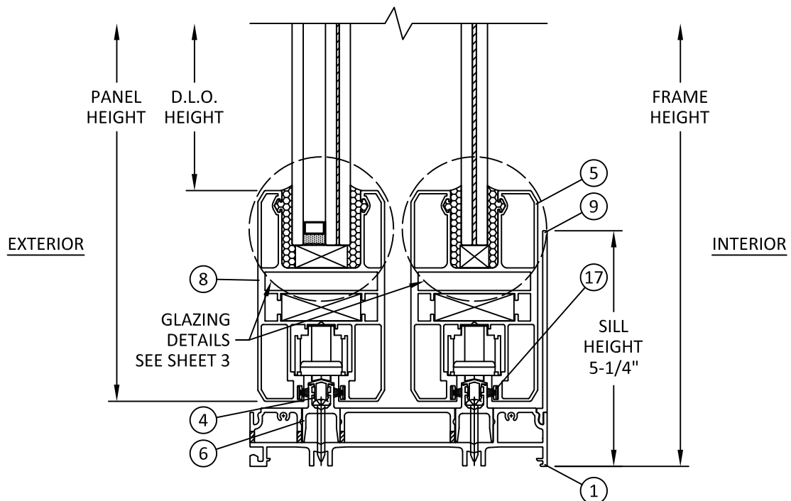
B 5 VERTICAL SECTION 2-TRACK SILL
