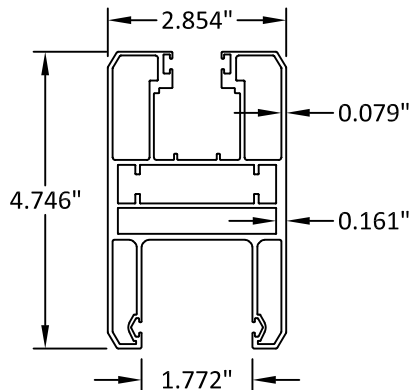
8 PANEL RAIL/STILE (INS.)
