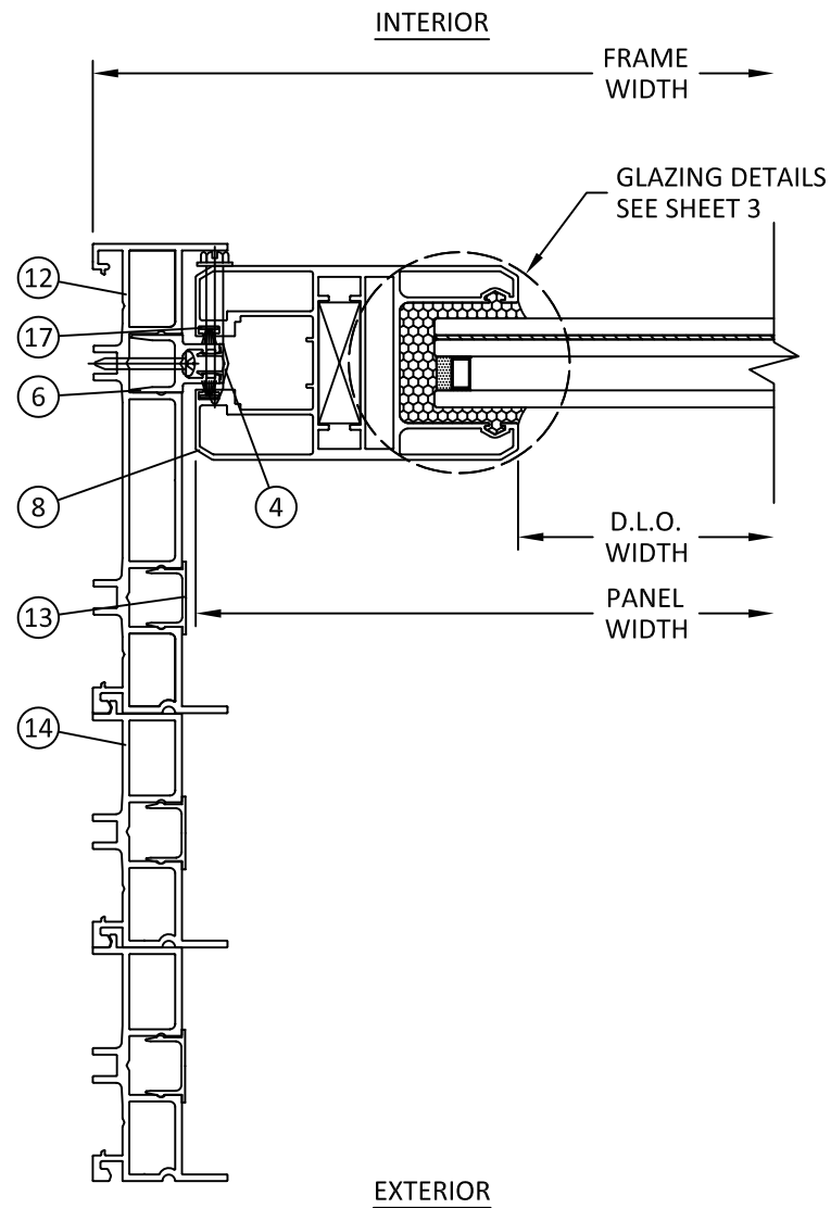
L 8 HORIZONTAL SECTION 4-TRACK JAMB FIXED PANEL
