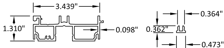
10 3/4 TRACK ADAPTER HEAD/SILL
