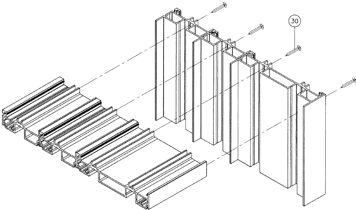
FRAME CORNER DETAIL 4 TRACK FRAME
