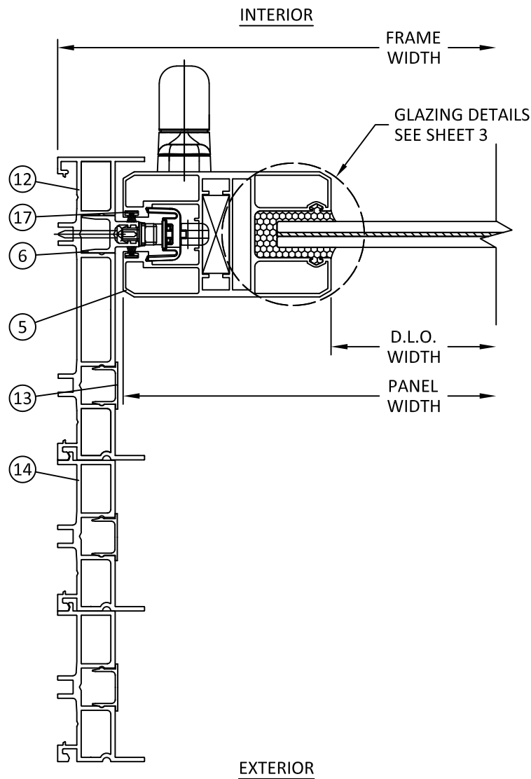
K 8 HORIZONTAL SECTION 4-TRACK JAMB OPERABLE PANEL
